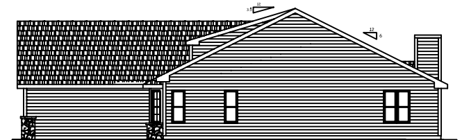
Left Elevation
