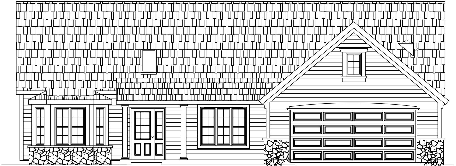
Front Elevation
