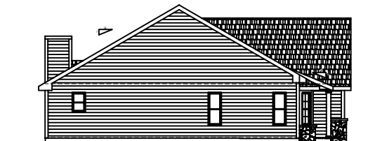
Left Elevation
