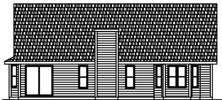
Rear Elevation
