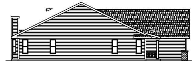
Left Elevation
